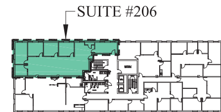
SECOND FLOOR KEY PLAN
